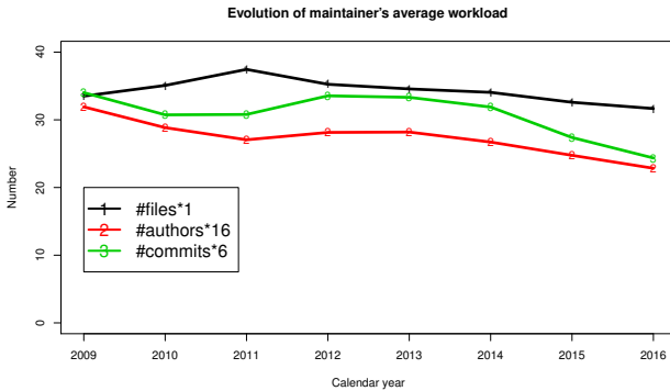
Figure 10: Average workload per maintainer
