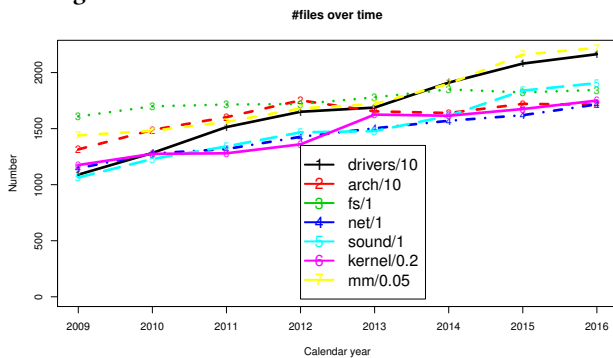
Figure 3: Numbers of maintained files in different modules
